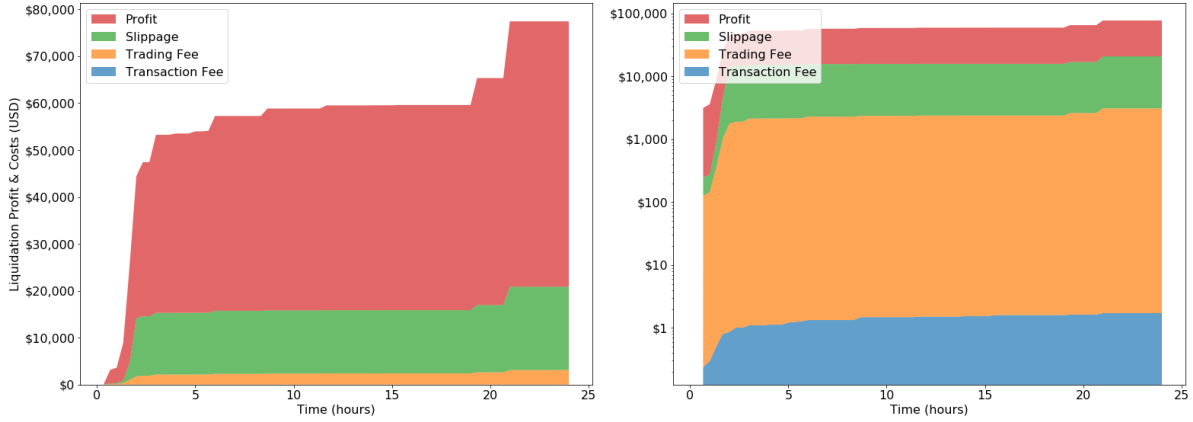
(a) 3% daily volatility
