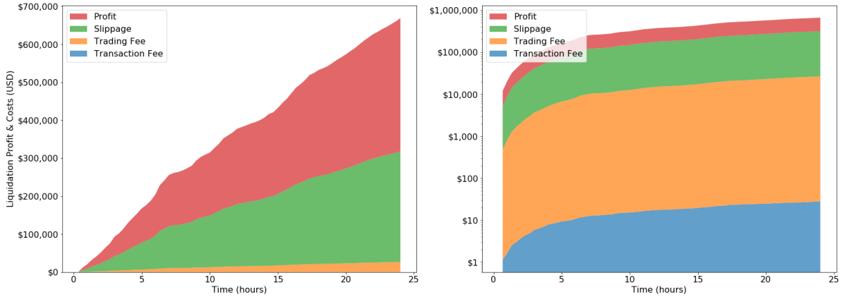
(b) 50% daily volatility
